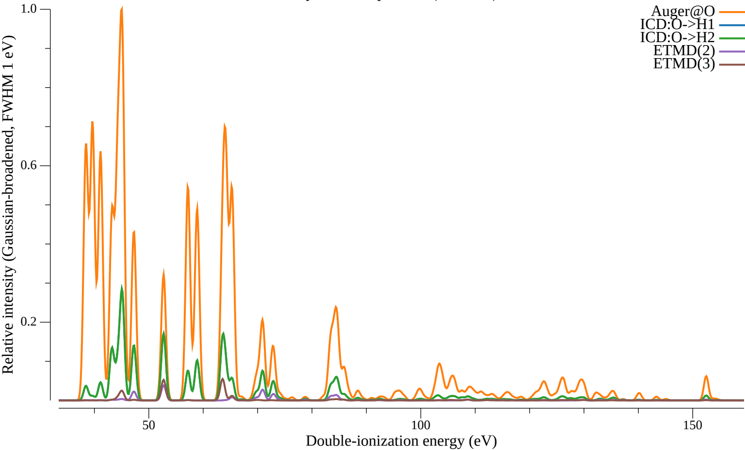
h2o Decay-channel spectrum (initial: O)
