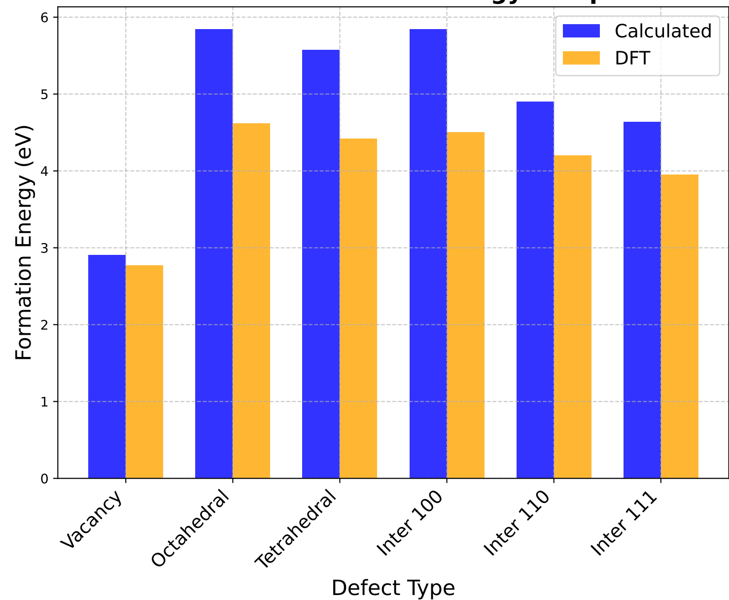
Point Defects Formation Energy Comparison
