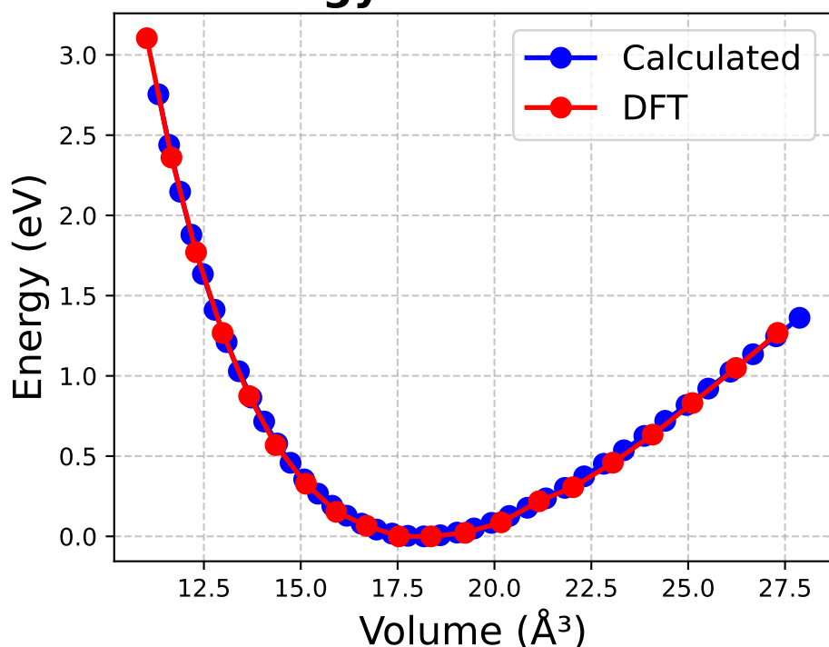
Energy-Volume Curve
