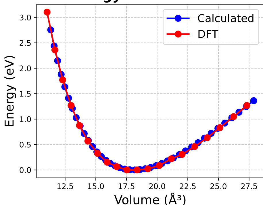
Energy-Volume Curve
