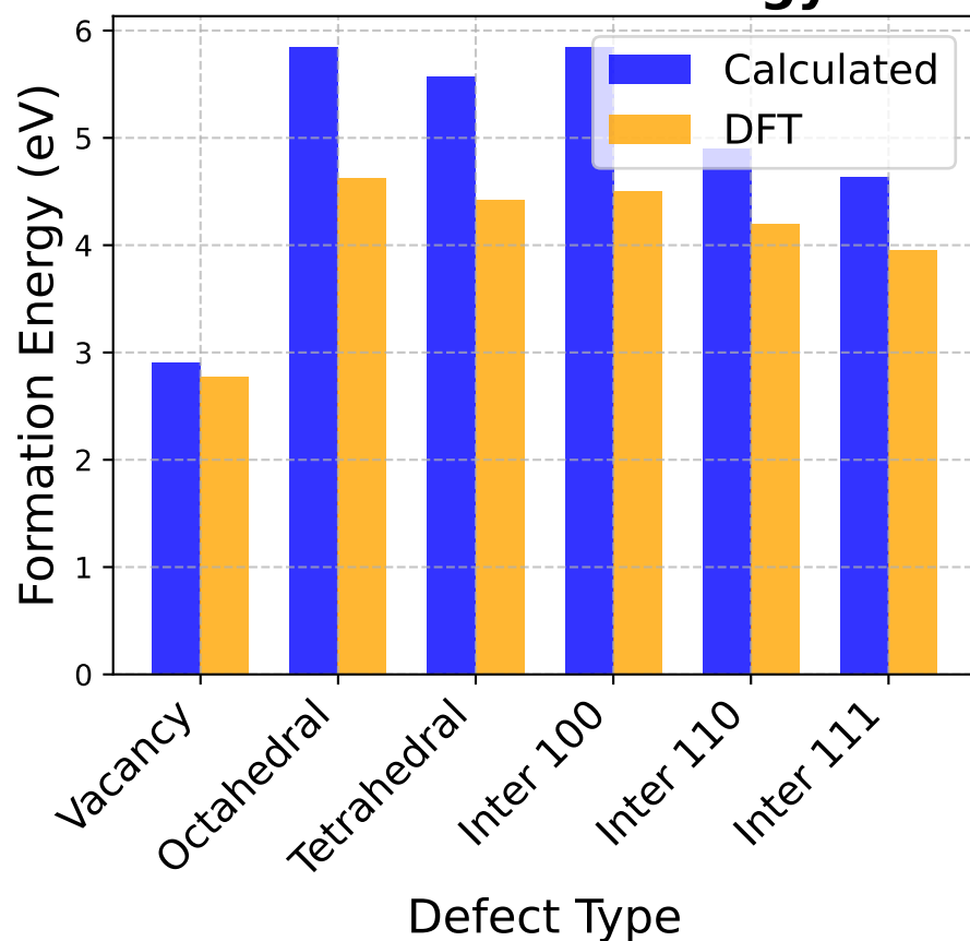
Point Defects Formation Energy Comparison
