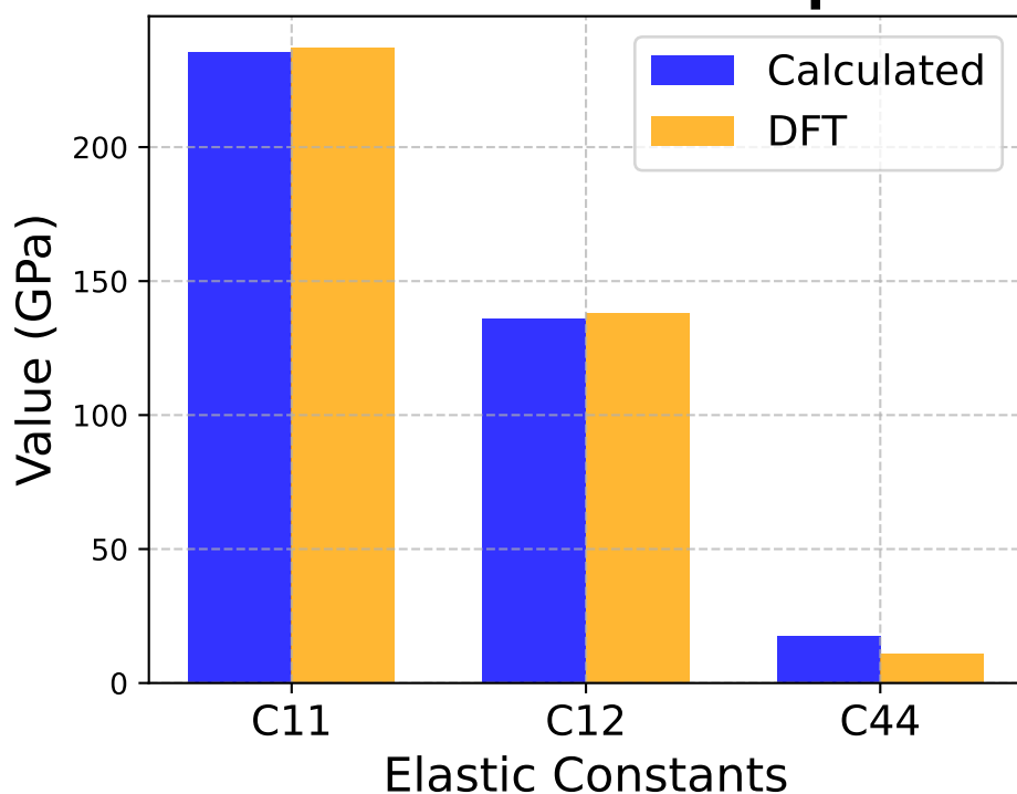
Elastic Constants Comparison
