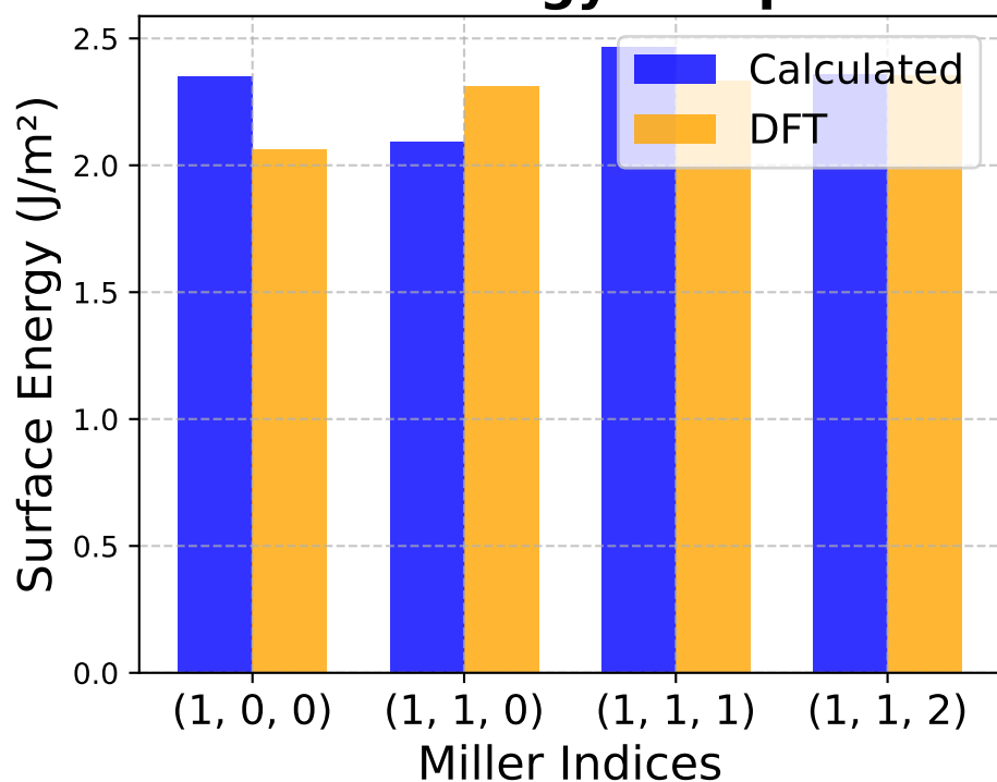
Surface Energy Comparison
