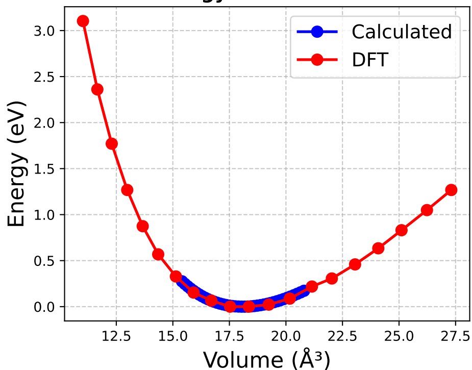
Energy-Volume Curve
