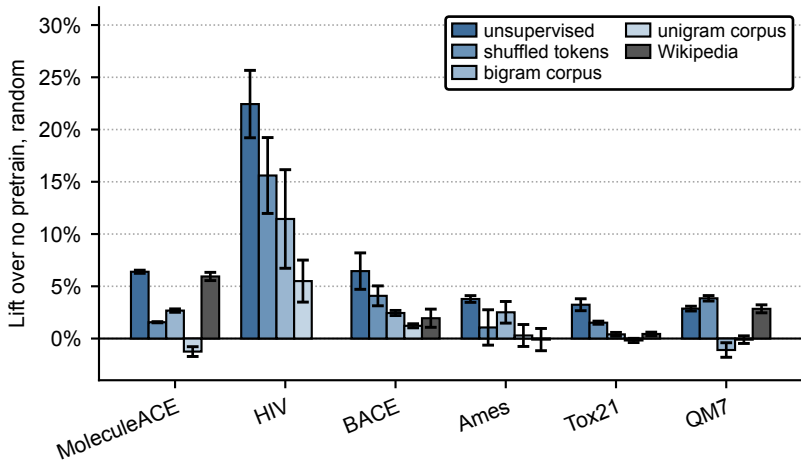
b Unsupervised: degraded corpus statistics
