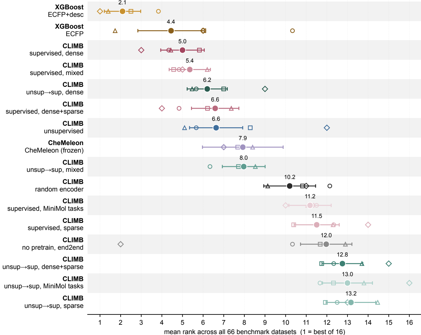
Overall standing across every benchmark (66 datasets, 4 suites)
