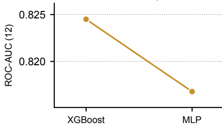
Tox21 ↑
