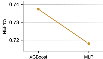
Tox21 ↑
