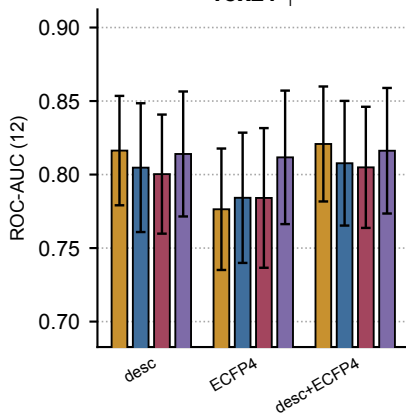
Tox21 ↑
