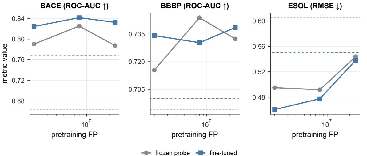
Fig E1 (H5) — is the flat ladder a frozen-probe artifact?
