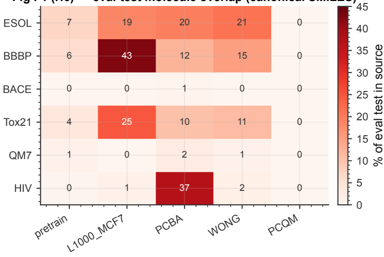
Fig F1 (H6) — eval-test molecule overlap (canonical SMILES)
