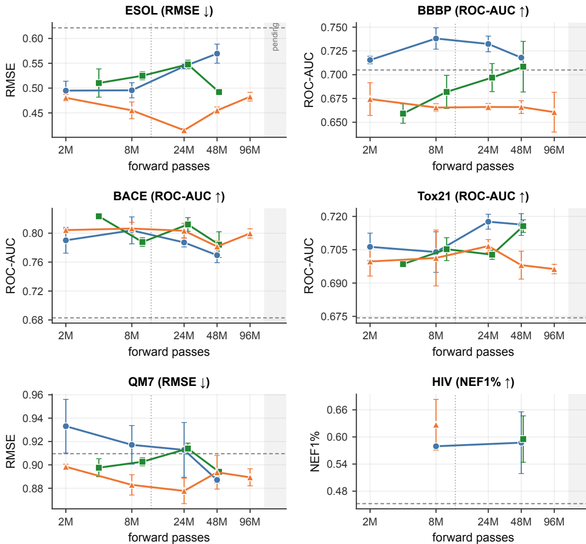
Fig A2 - scaling of the primary regimes in pretraining compute
