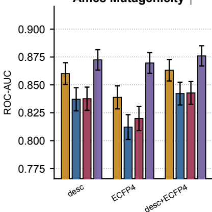
Ames Mutagenicity ↑
