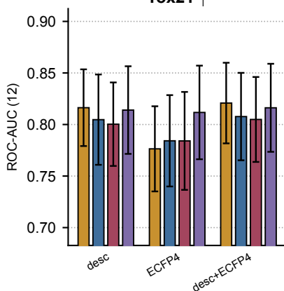
Tox21 ↑
