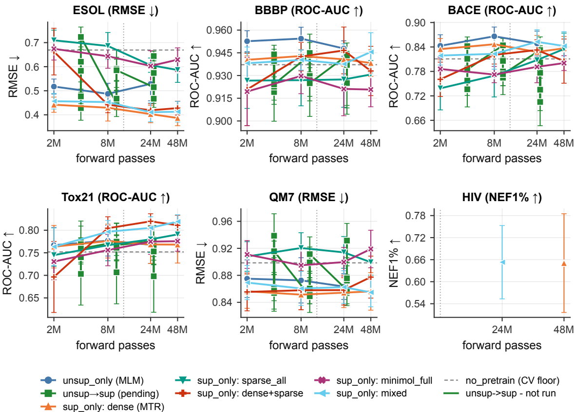
Fig A2 (H1+H4) - scaling of unsup_only vs sup_only (frozen probe, scaffold 5-fold CV; bars = fold std)
