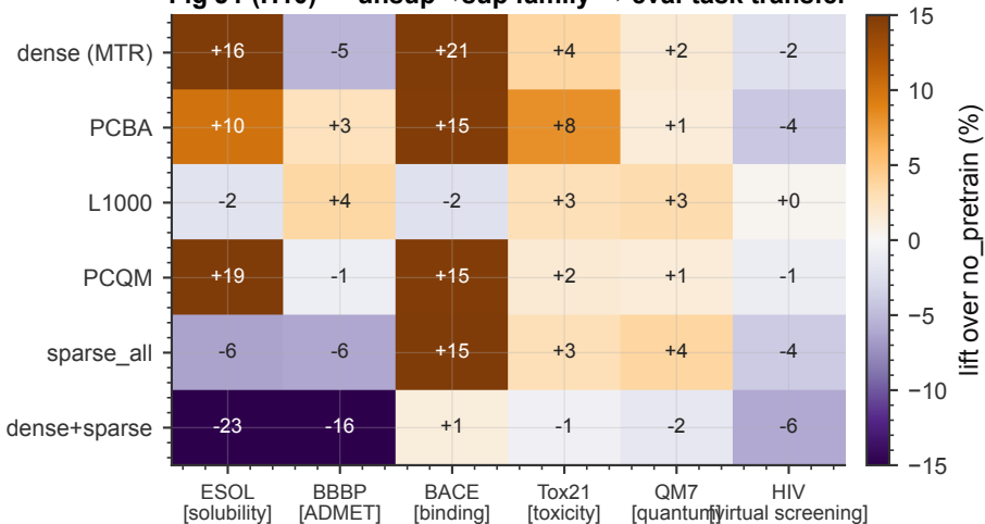
Fig J1 (H10) — unsup→sup family → eval-task transfer
