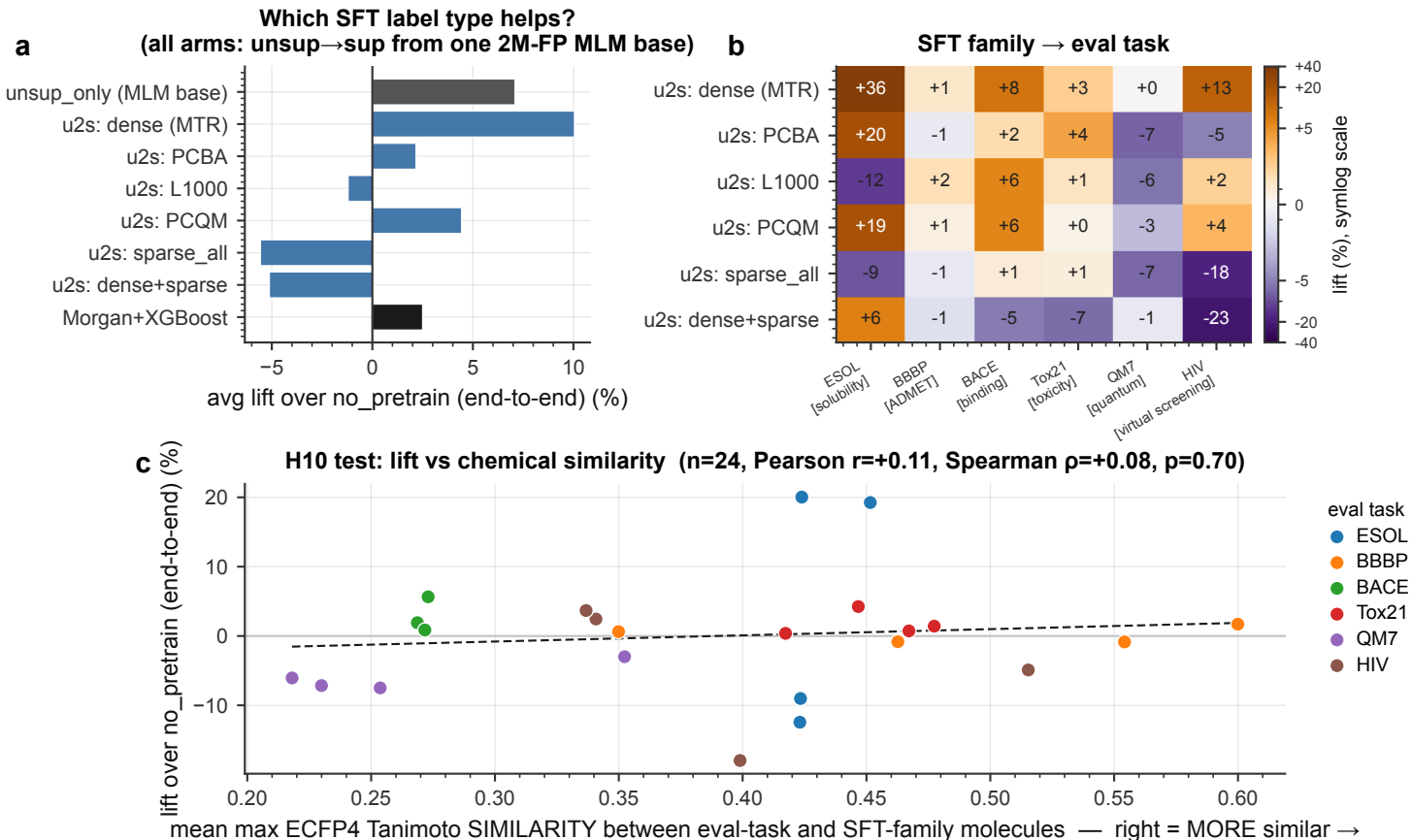
Fig C1J1 - supervised pretraining data: which type helps, how much, and does it follow chemistry?
