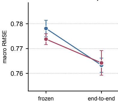
Ames GeneTox ↑
