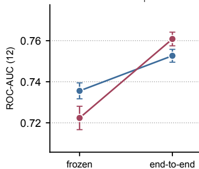
Tox21 ↑
