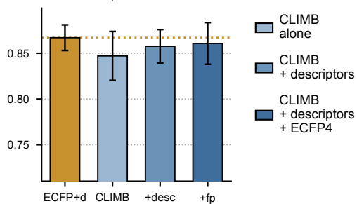
h QM7 ↓
