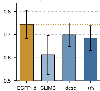
g Tox21 ↑
