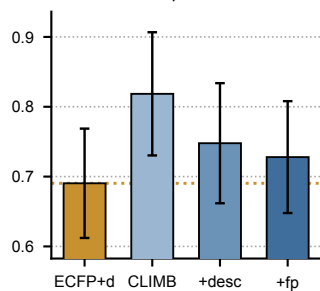
f Ames ↑
