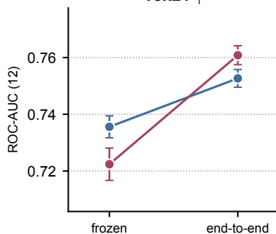
Tox21 ↑
