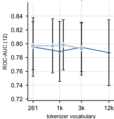
Tox21 ↑
