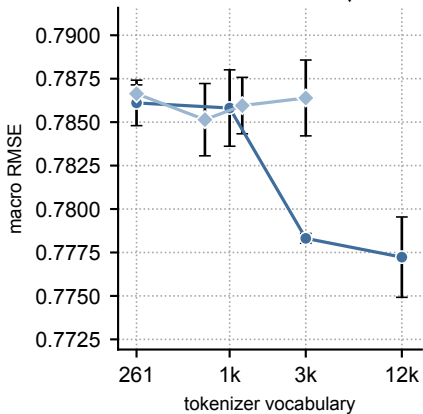
Ames Mutagenicity ↑
