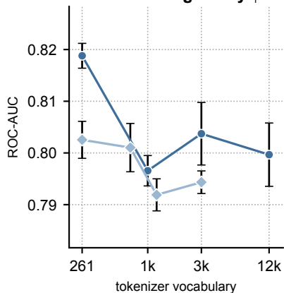
Ames Mutagenicity ↑
