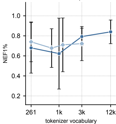
Tox21 ↑
