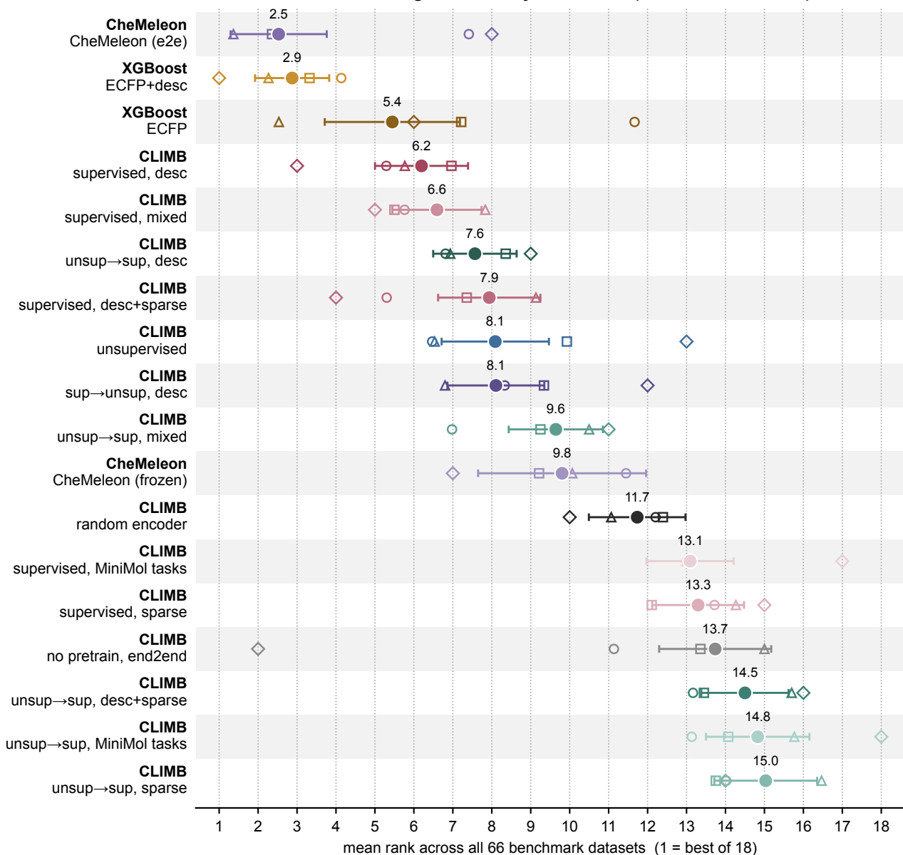
Overall standing across every benchmark (66 datasets, 4 suites)
