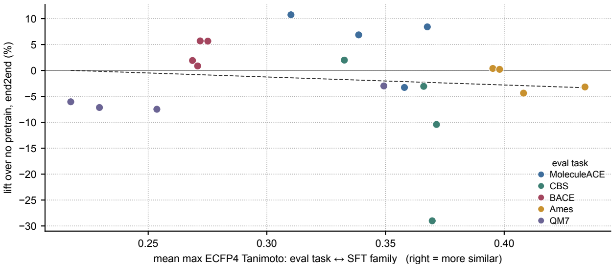
Fig C2 — Supervised pretraining: transfer vs chemical similarity (n=20, Pearson r=-0.11 , Spearman \rho=-0.11 , p=0.645 )
