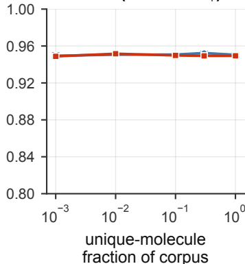
QM7 (RMSE ↓)
