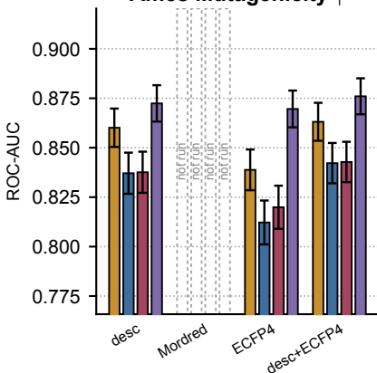
Ames Mutagenicity ↑
