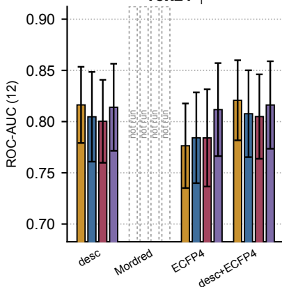
Tox21 ↑
