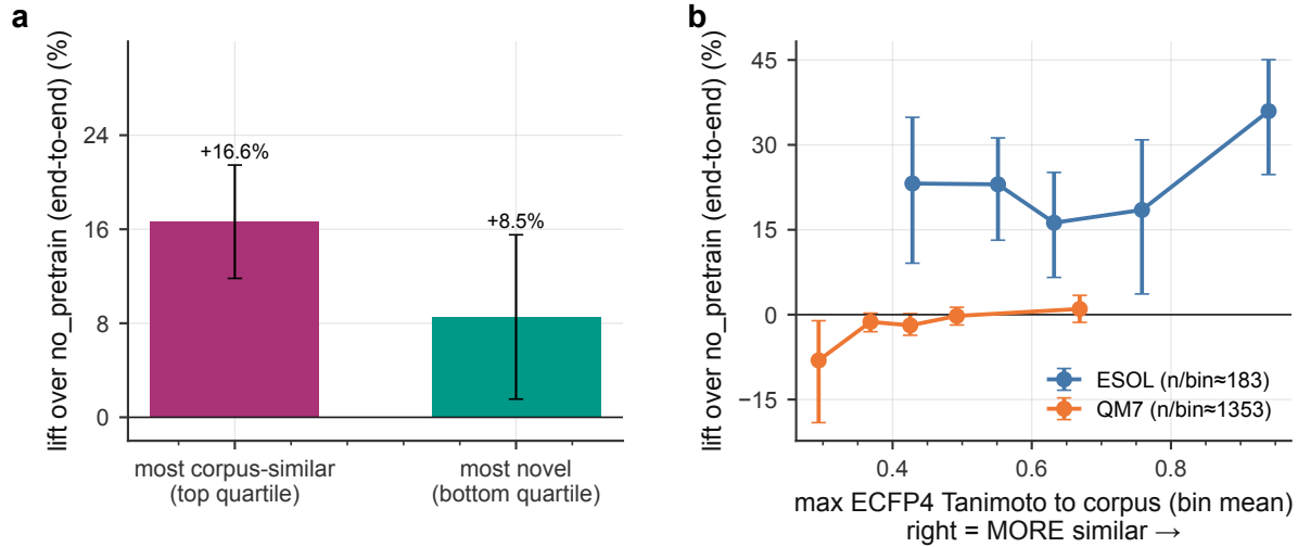
Fig I1 - memorization or representation? Who benefits from MLM pretraining
