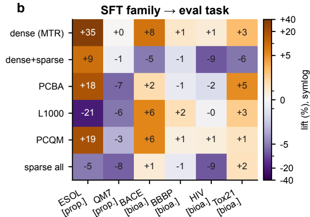
Fig D — Task similarity between supervised pretraining and downstream task
