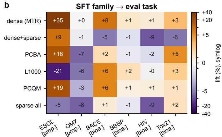
Fig D — Task similarity between supervised pretraining and downstream task
