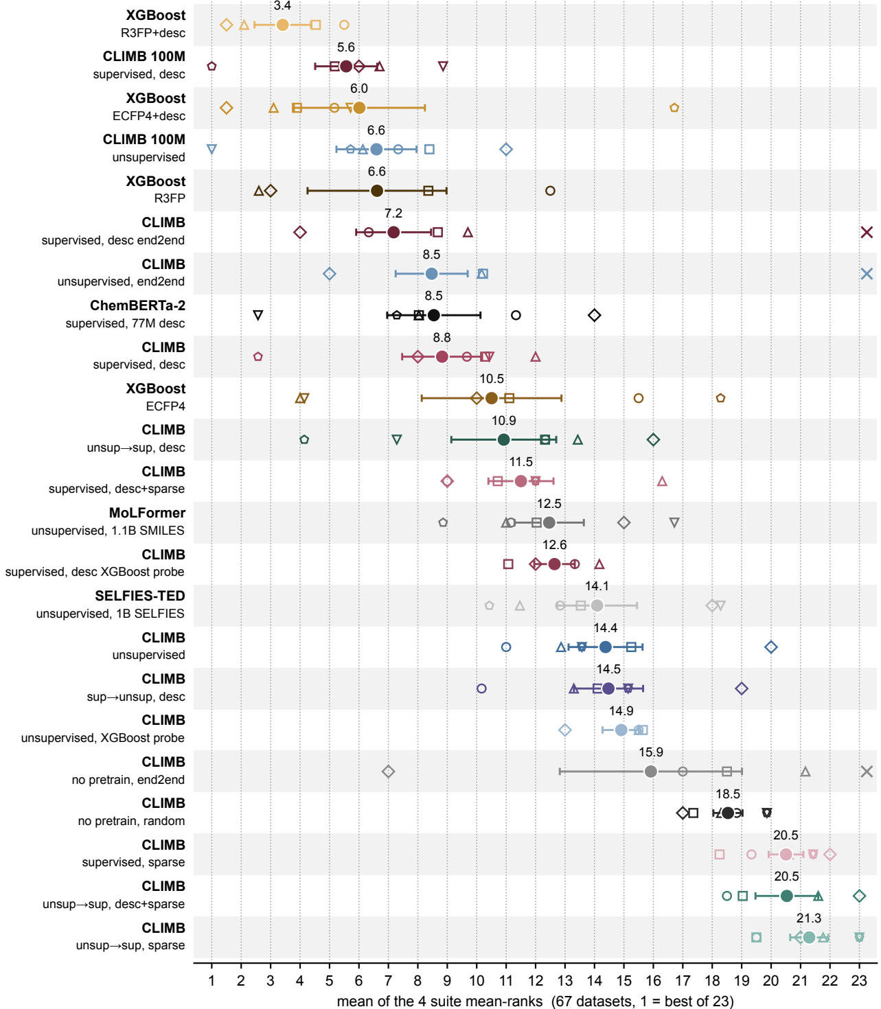
Overall standing: mean of the 4 suite ranks (67 datasets)
