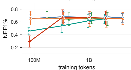
HIV (NEF1% ↑)
