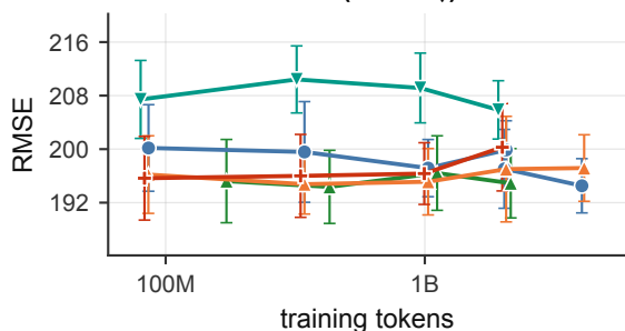
QM7 (RMSE ↓)
