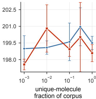
QM7 (RMSE ↓)
