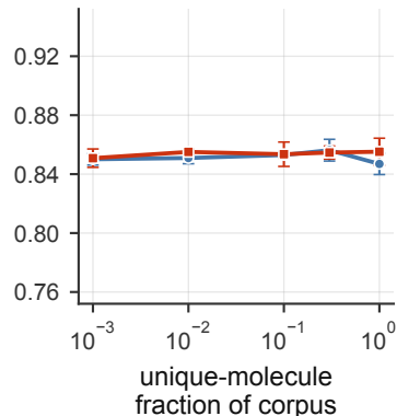
HIV (NEF1% ↑)
