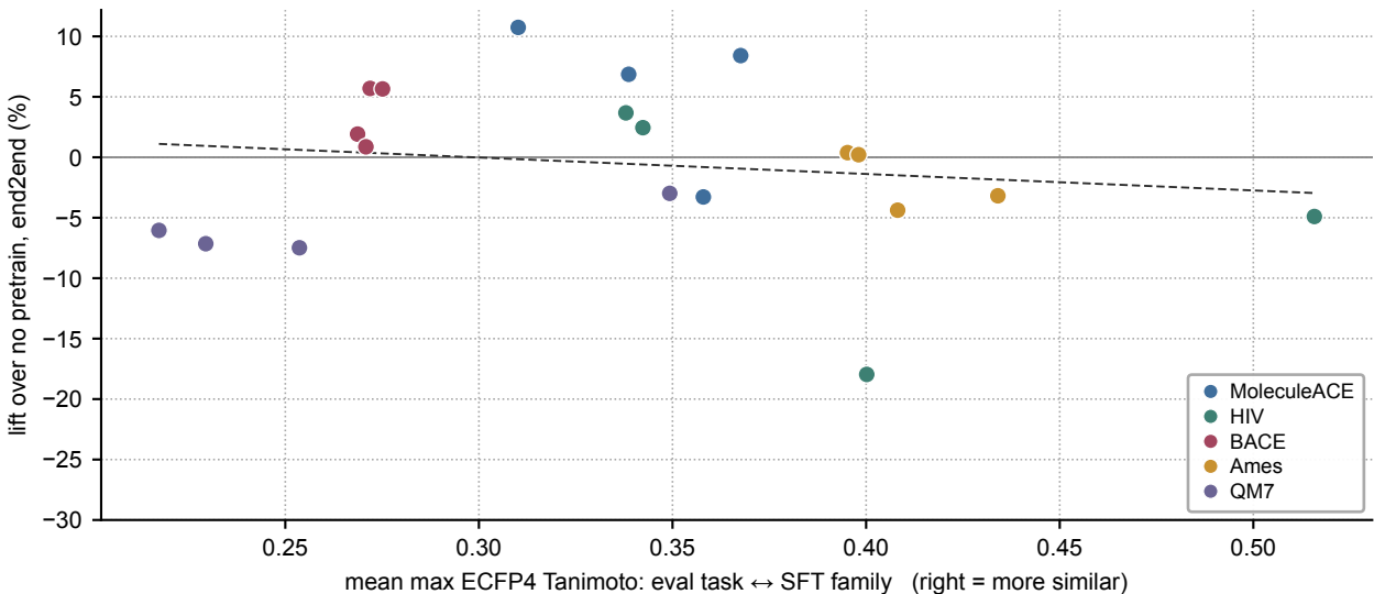
Fig C2 — Supervised pretraining: transfer vs chemical similarity (n=20, Pearson r=-0.15 , Spearman \rho=-0.10 , p=0.673 )
