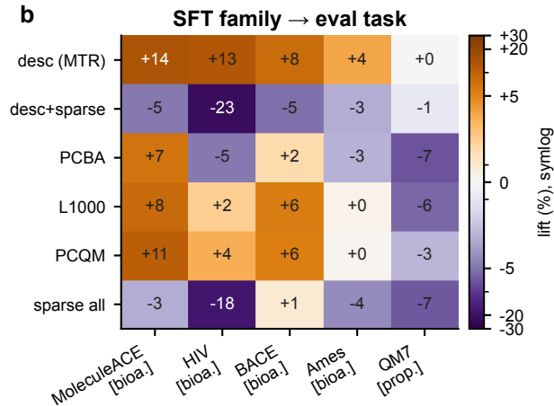
Fig D — Task similarity between supervised pretraining and downstream task
