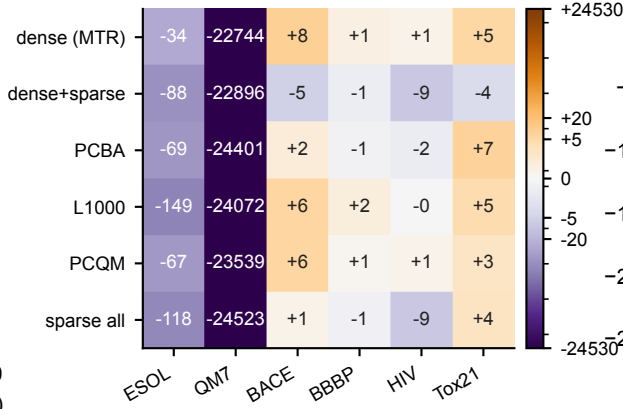
e SFT family → eval task
