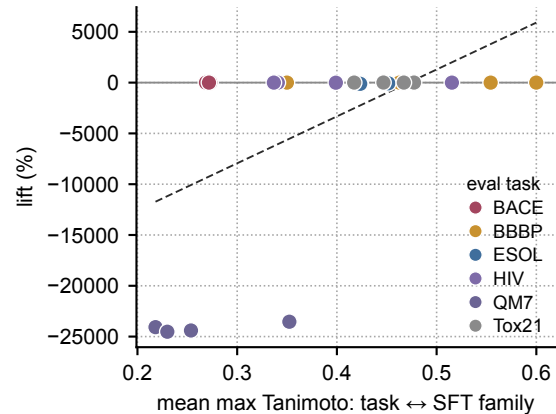
f Descriptor-like task mapping
