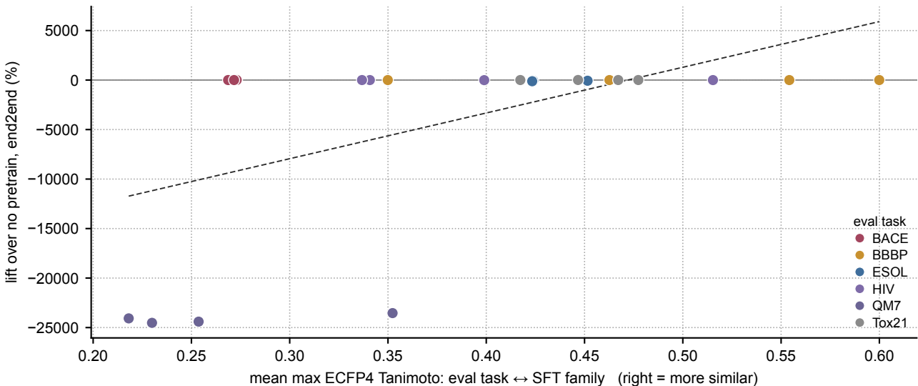
Fig C2 — Supervised pretraining: transfer vs chemical similarity (n=24, Pearson r=+0.53 , Spearman \rho=+0.22 , p=0.296 )
