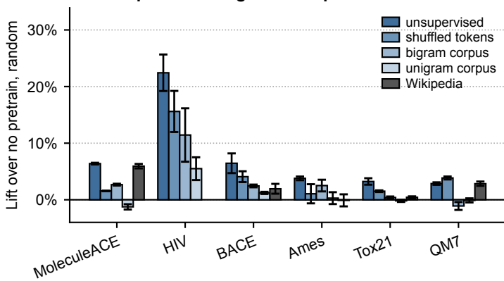
e BACE ↑
