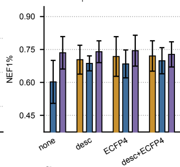
g Tox21 ↑
