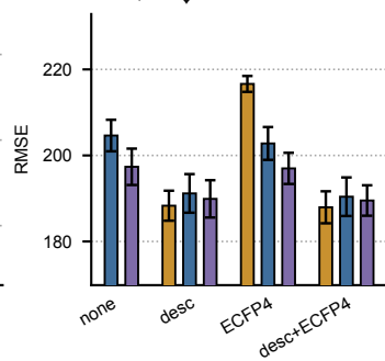
h QM7 ↓
