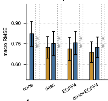
f Ames ↑
