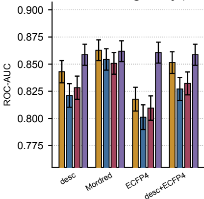
Ames Mutagenicity ↑
