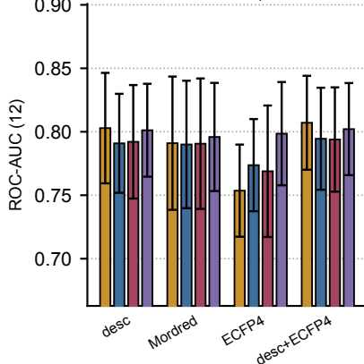
Tox21 ↑
