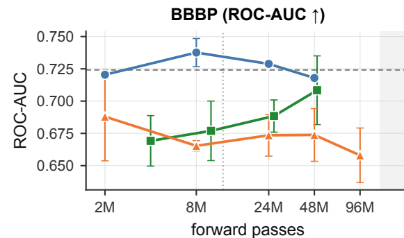
Fig A2 - scaling of the primary regimes in pretraining compute
