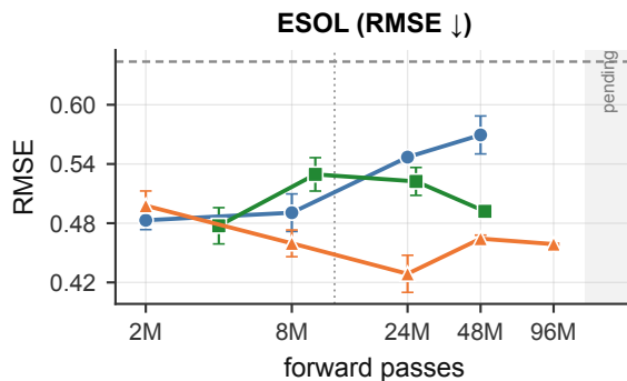
Fig A2 - scaling of the primary regimes in pretraining compute
