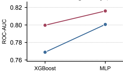
Ames Mutagenicity ↑
