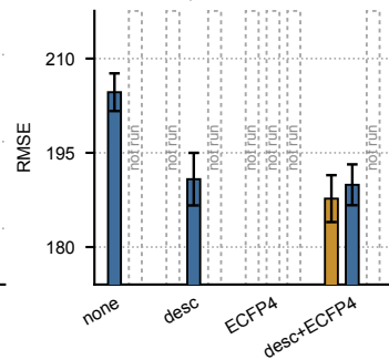
h QM7 ↓
