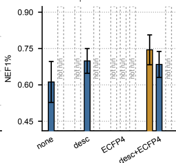
g Tox21 ↑
