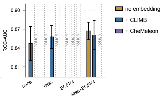
h QM7 ↓
