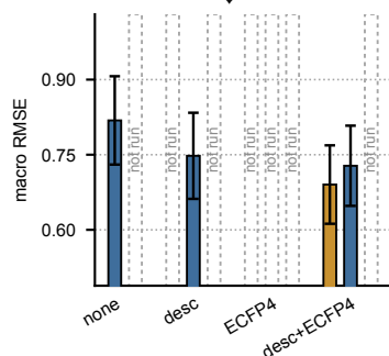
f Ames ↑
