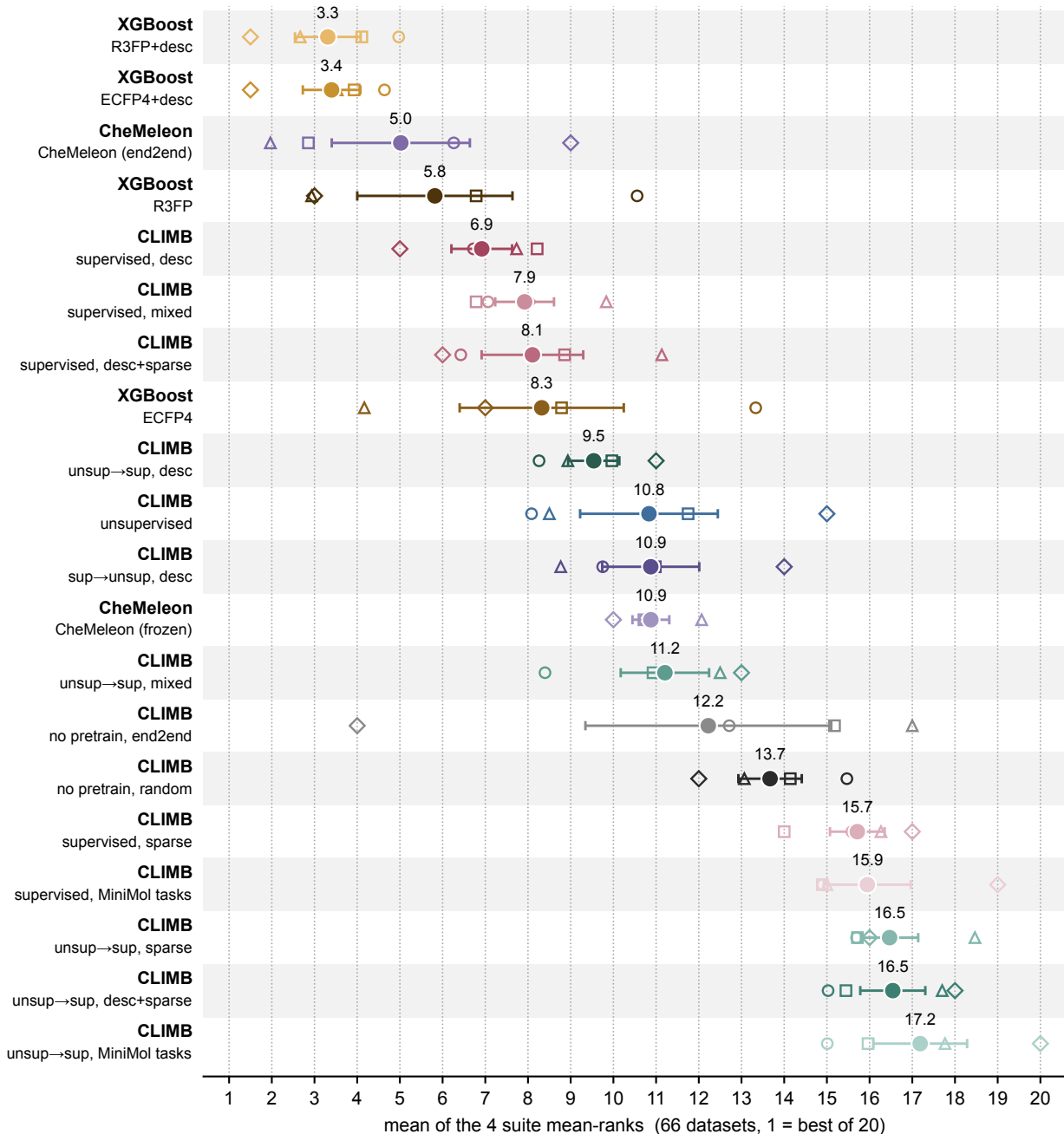
Overall standing: mean of the 4 suite ranks (66 datasets)
