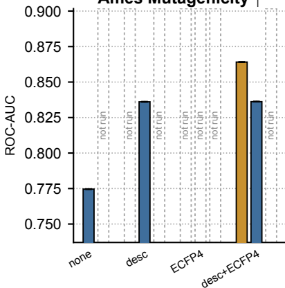
Ames Mutagenicity ↑
