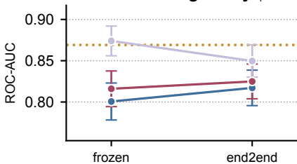
Ames Mutagenicity ↑
