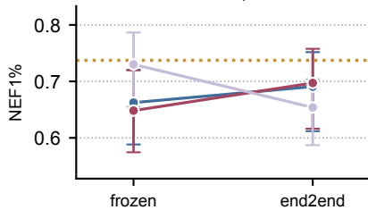
Tox21 ↑
