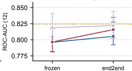
Tox21 ↑
