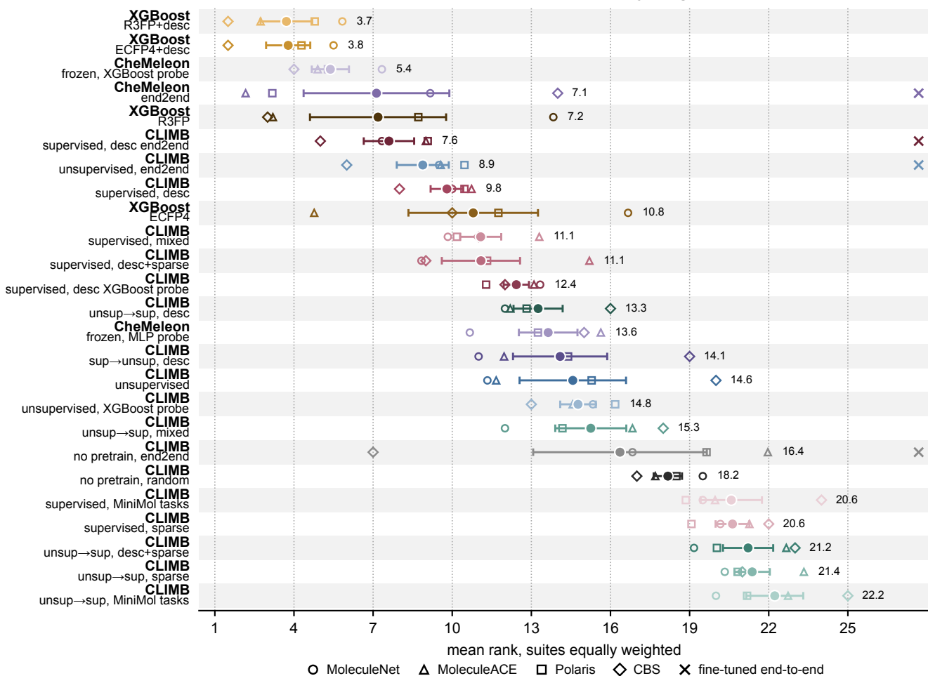
Mean rank, four suites equally weighted
