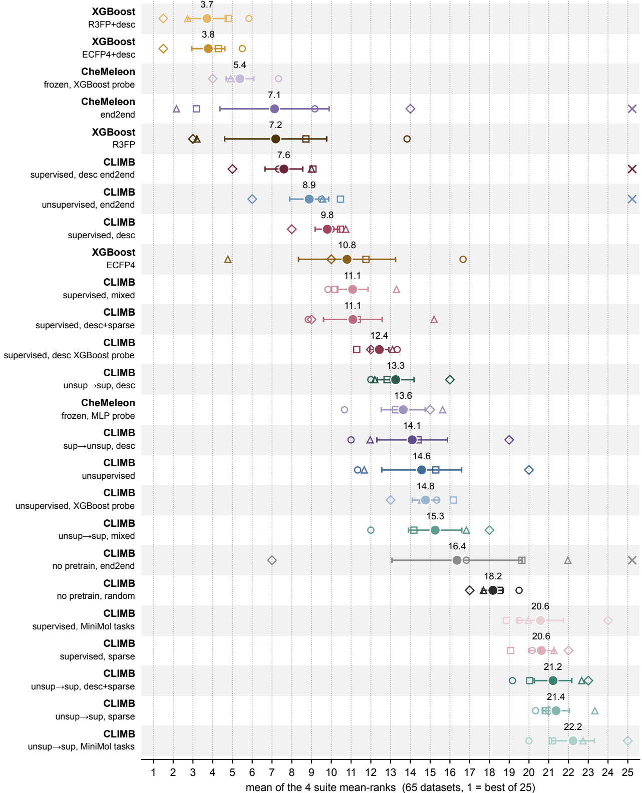
Overall standing: mean of the 4 suite ranks (65 datasets)
