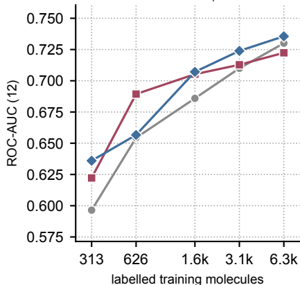
Tox21 ↑
