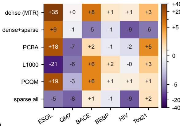
e SFT family → eval task
