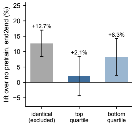
a Lift by similarity group
