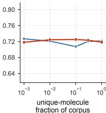
QM7 (RMSE ↓)
