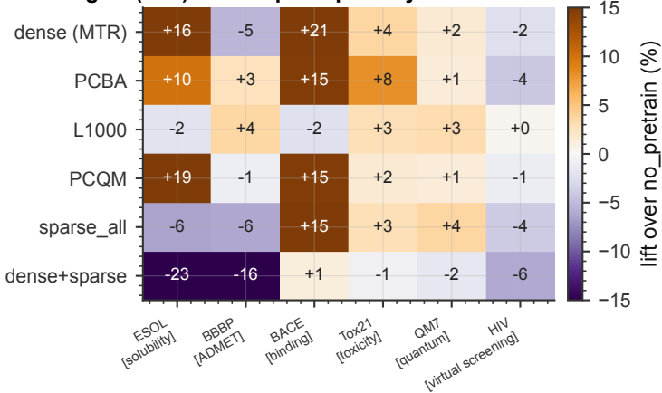
Fig J1 (H10) — unsup→sup family → eval-task transfer
