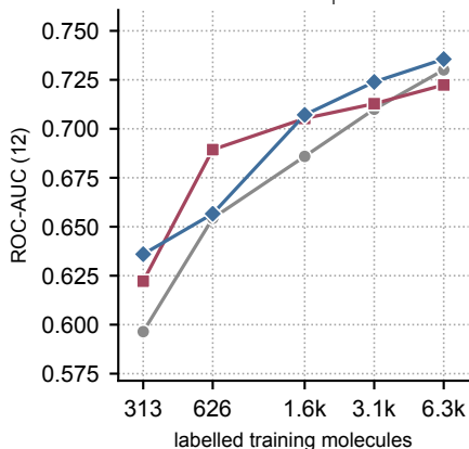
Tox21 ↑
