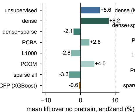
d Lift by SFT label type
